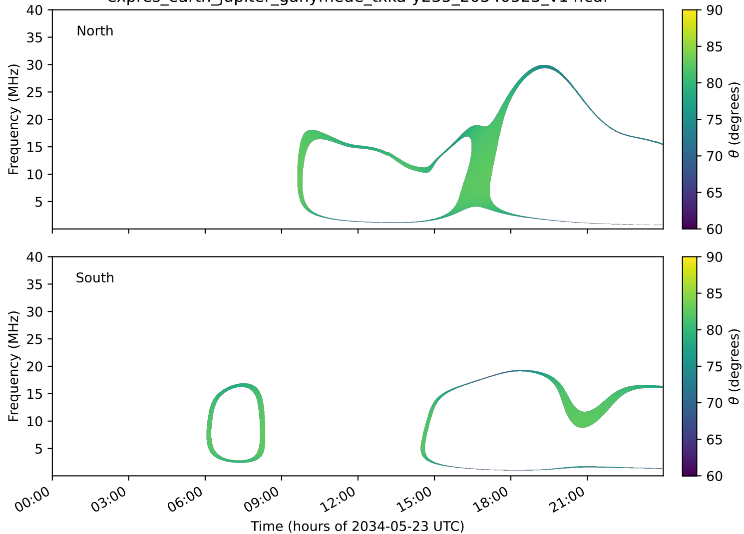
expres_earth_jupiter_ganymede_txka-y235_20340523_v14.cdf
