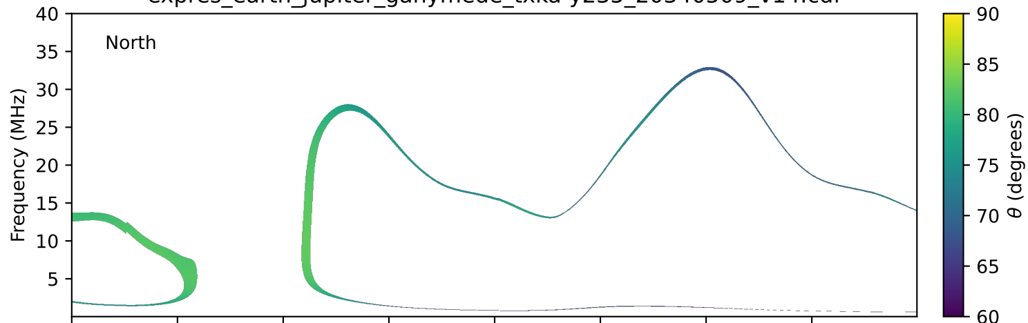
expres_earth_jupiter_ganymede_txka-y235_20340509_v14.cdf
