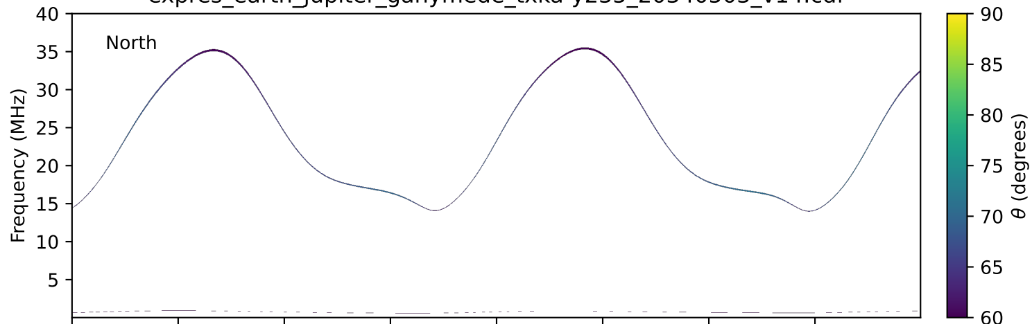
expres_earth_jupiter_ganymede_txka-y235_20340503_v14.cdf
