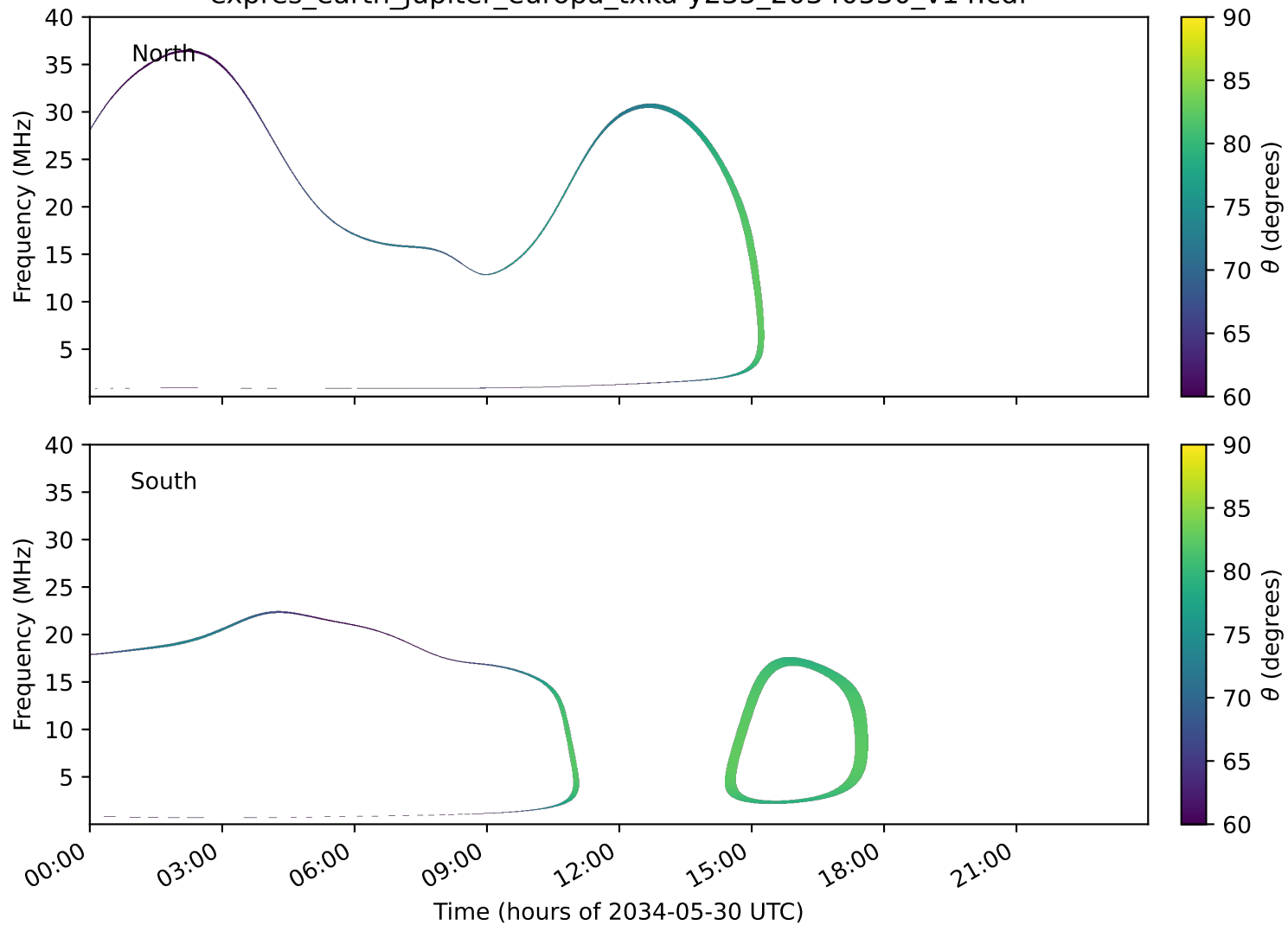
expres_earth_jupiter_europa_txka-y235_20340530_v14.cdf
