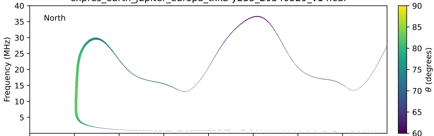
expres_earth_jupiter_europa_txka-y235_20340529_v14.cdf
