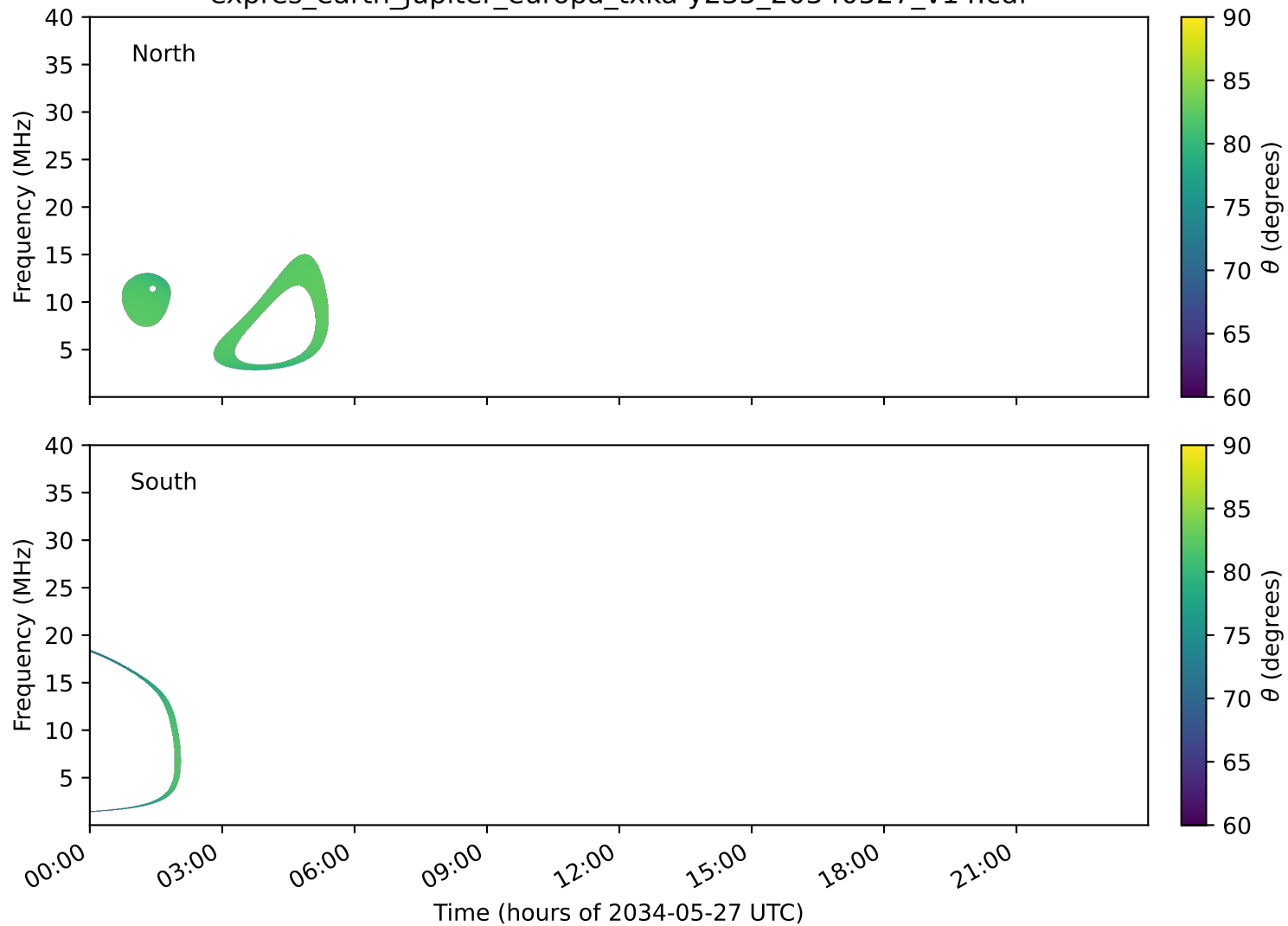
expres_earth_jupiter_europa_txka-y235_20340527_v14.cdf
