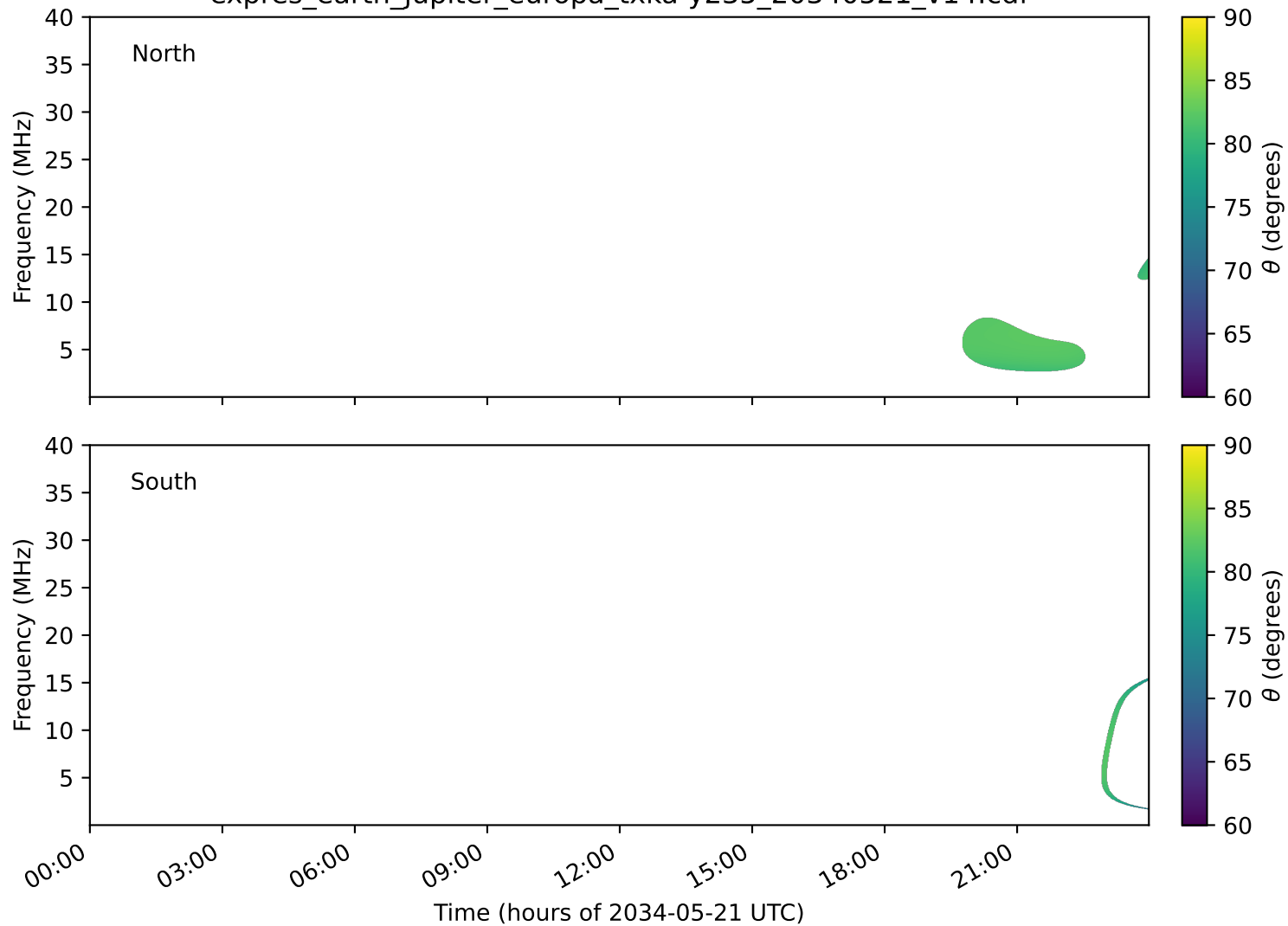
expres_earth_jupiter_europa_txka-y235_20340521_v14.cdf
