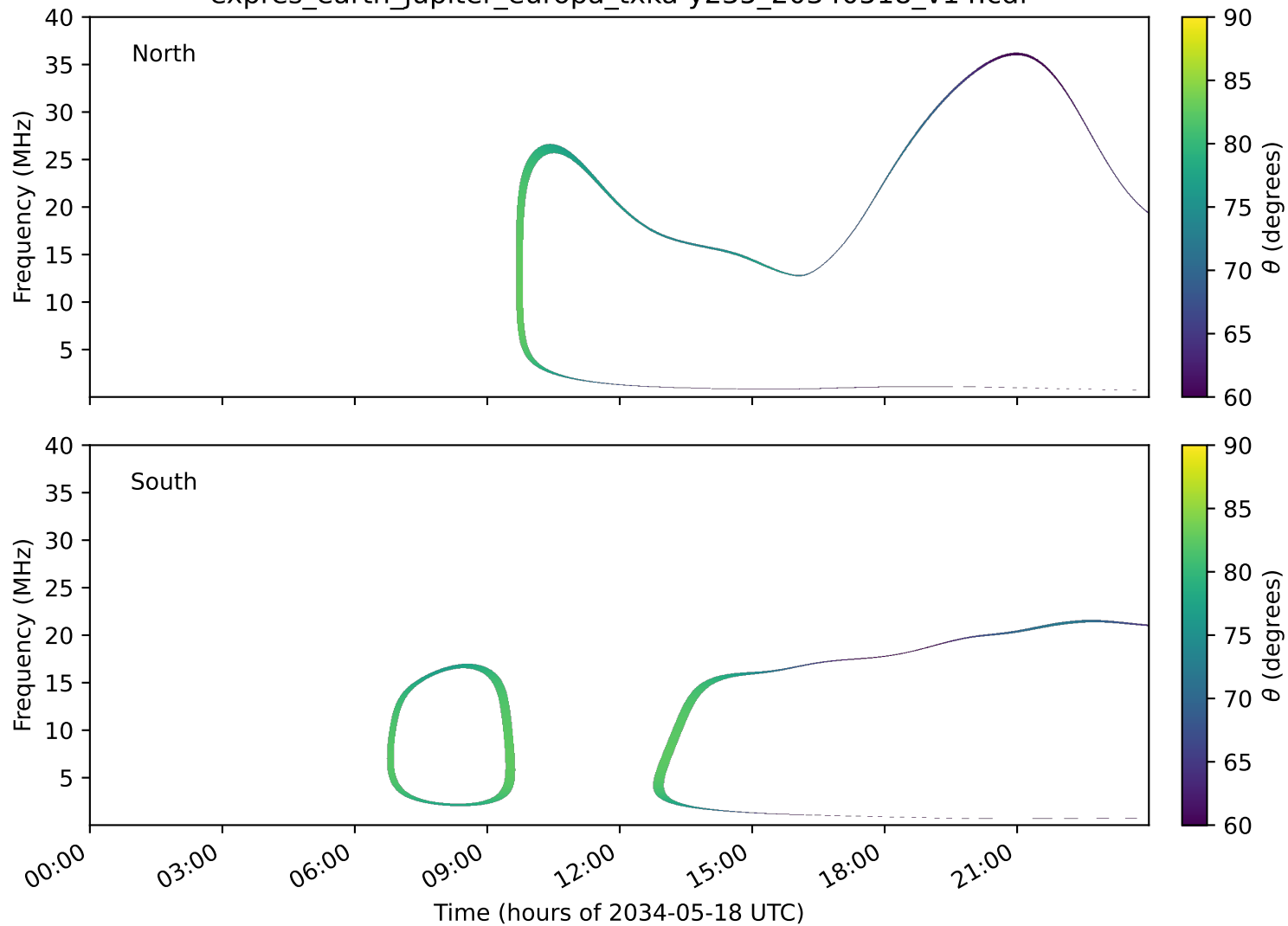
expres_earth_jupiter_europa_txka-y235_20340518_v14.cdf
