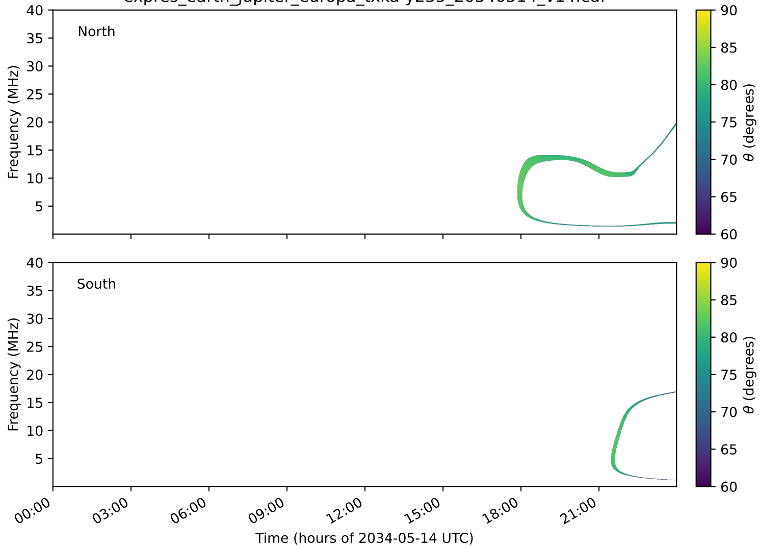
expres_earth_jupiter_europa_txka-y235_20340514_v14.cdf
