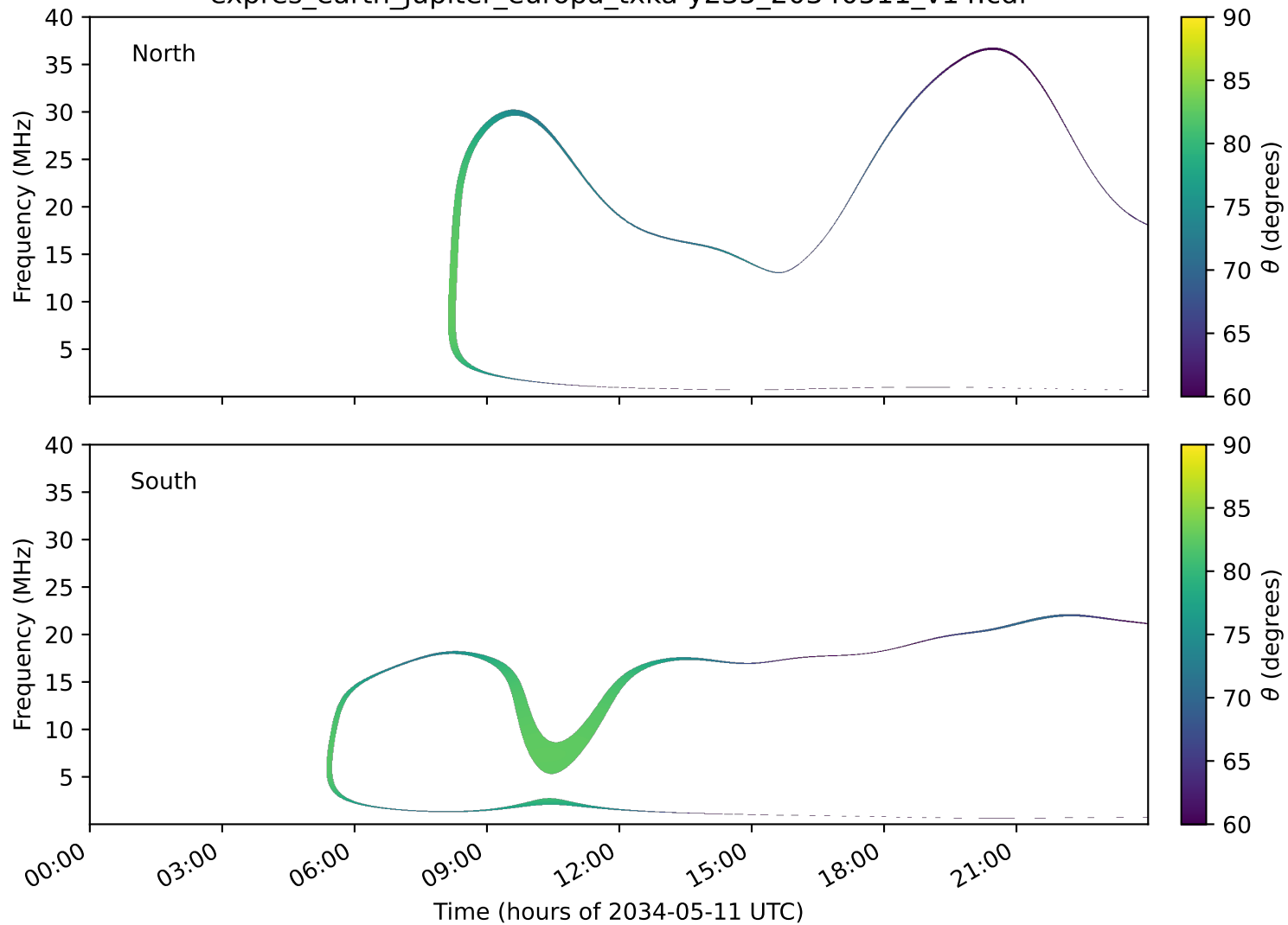
expres_earth_jupiter_europa_txka-y235_20340511_v14.cdf
