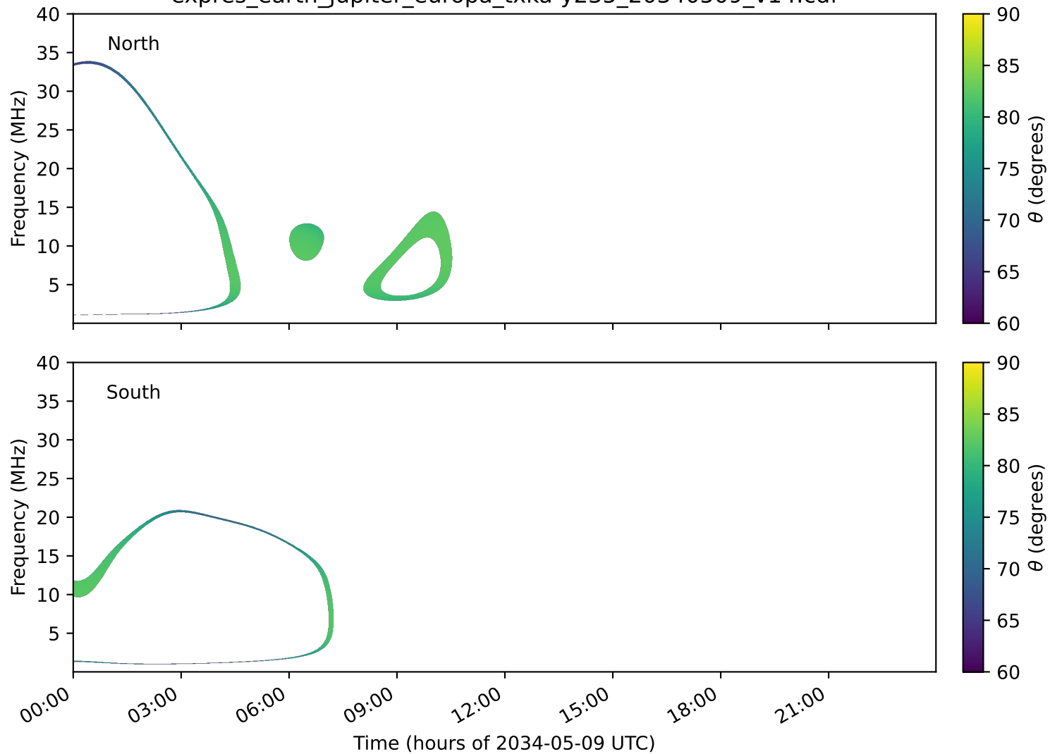
expres_earth_jupiter_europa_txka-y235_20340509_v14.cdf
