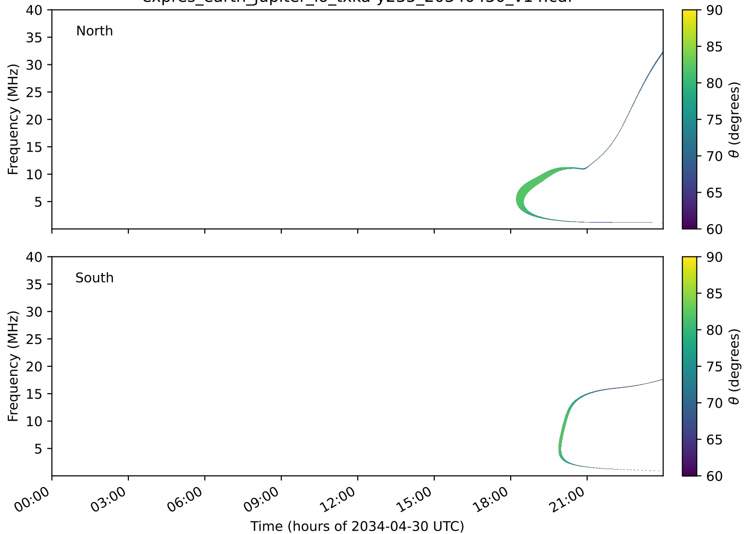
expres_earth_jupiter_io_txka-y235_20340430_v14.cdf
