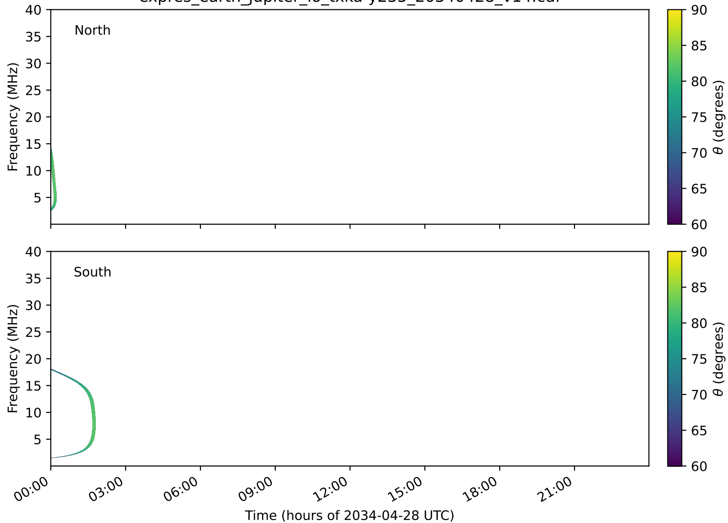
expres_earth_jupiter_io_txka-y235_20340428_v14.cdf
