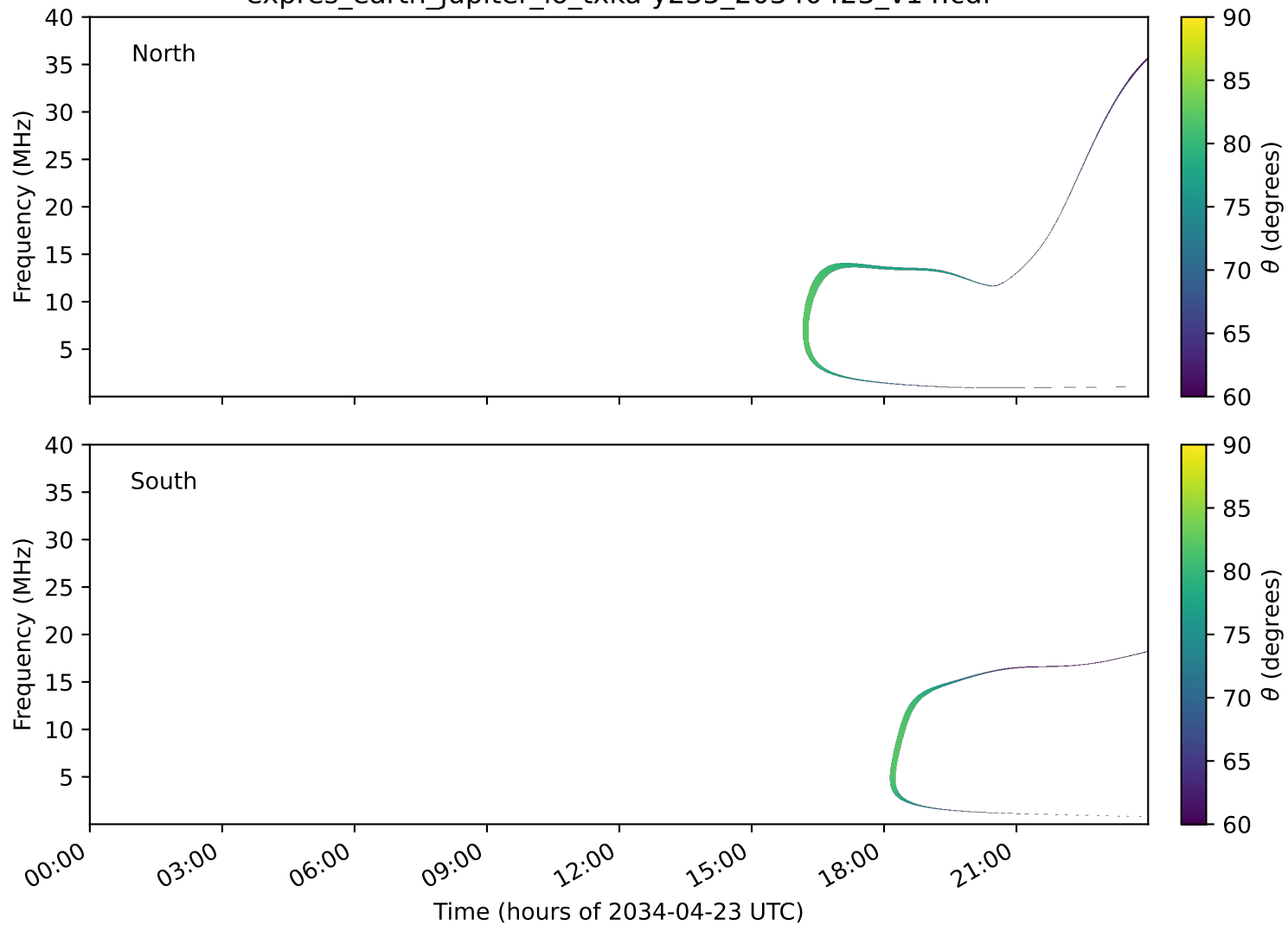
expres_earth_jupiter_io_txka-y235_20340423_v14.cdf
