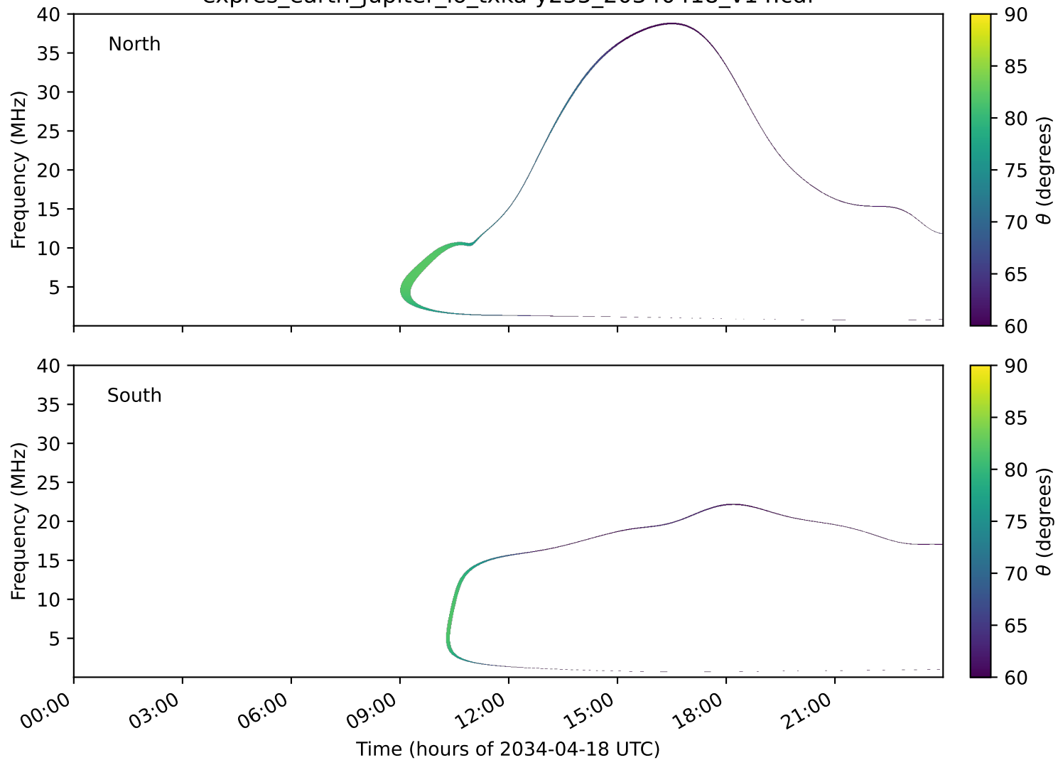
expres_earth_jupiter_io_txka-y235_20340418_v14.cdf
