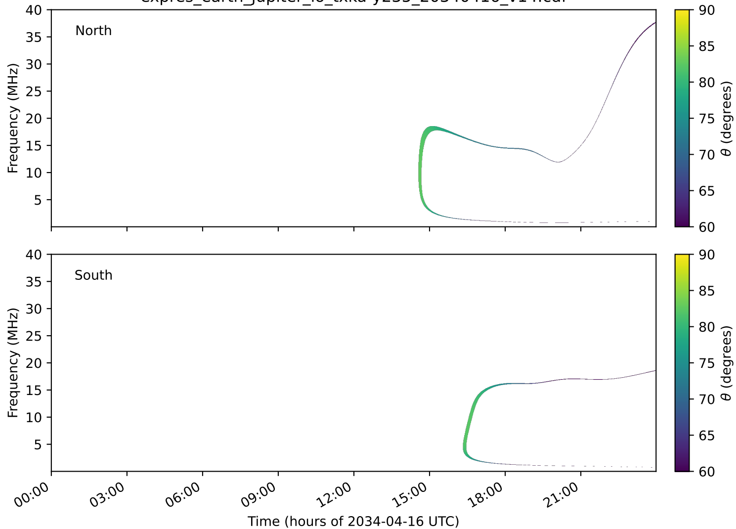
expres_earth_jupiter_io_txka-y235_20340416_v14.cdf
