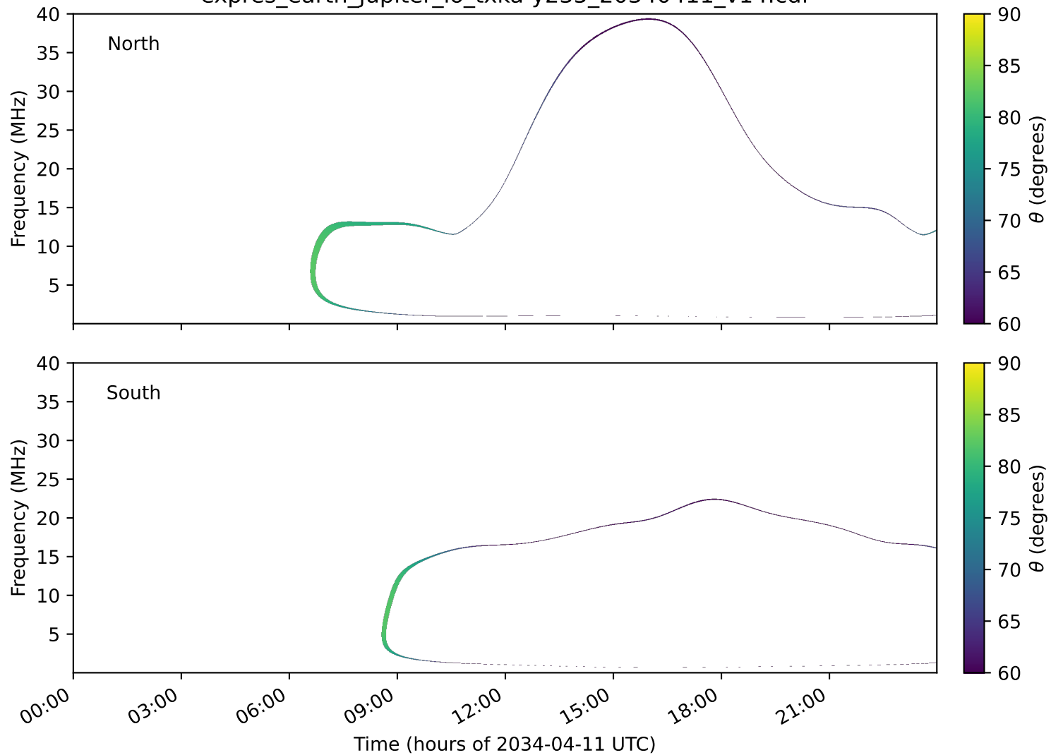
expres_earth_jupiter_io_txka-y235_20340411_v14.cdf
