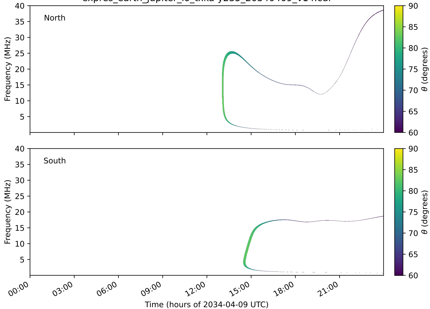
expres_earth_jupiter_io_txka-y235_20340409_v14.cdf
