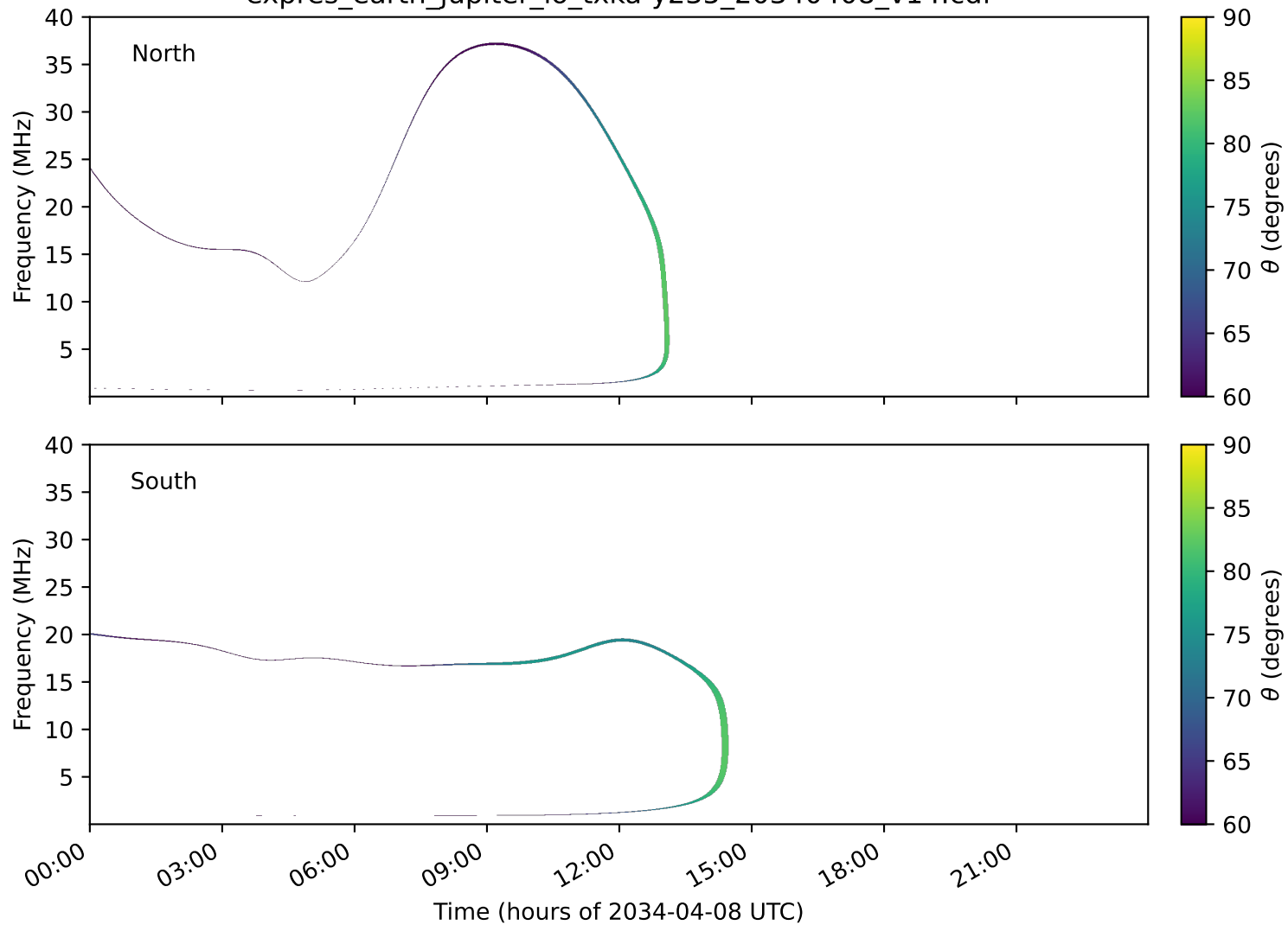
expres_earth_jupiter_io_txka-y235_20340408_v14.cdf
