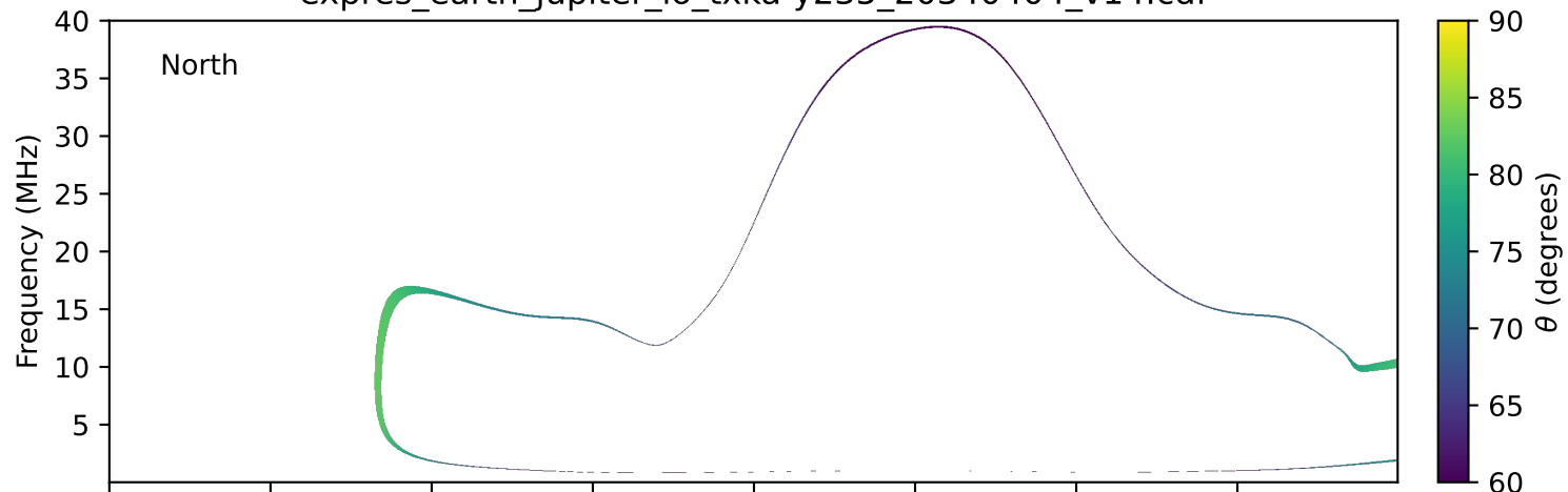
expres_earth_jupiter_io_txka-y235_20340404_v14.cdf
