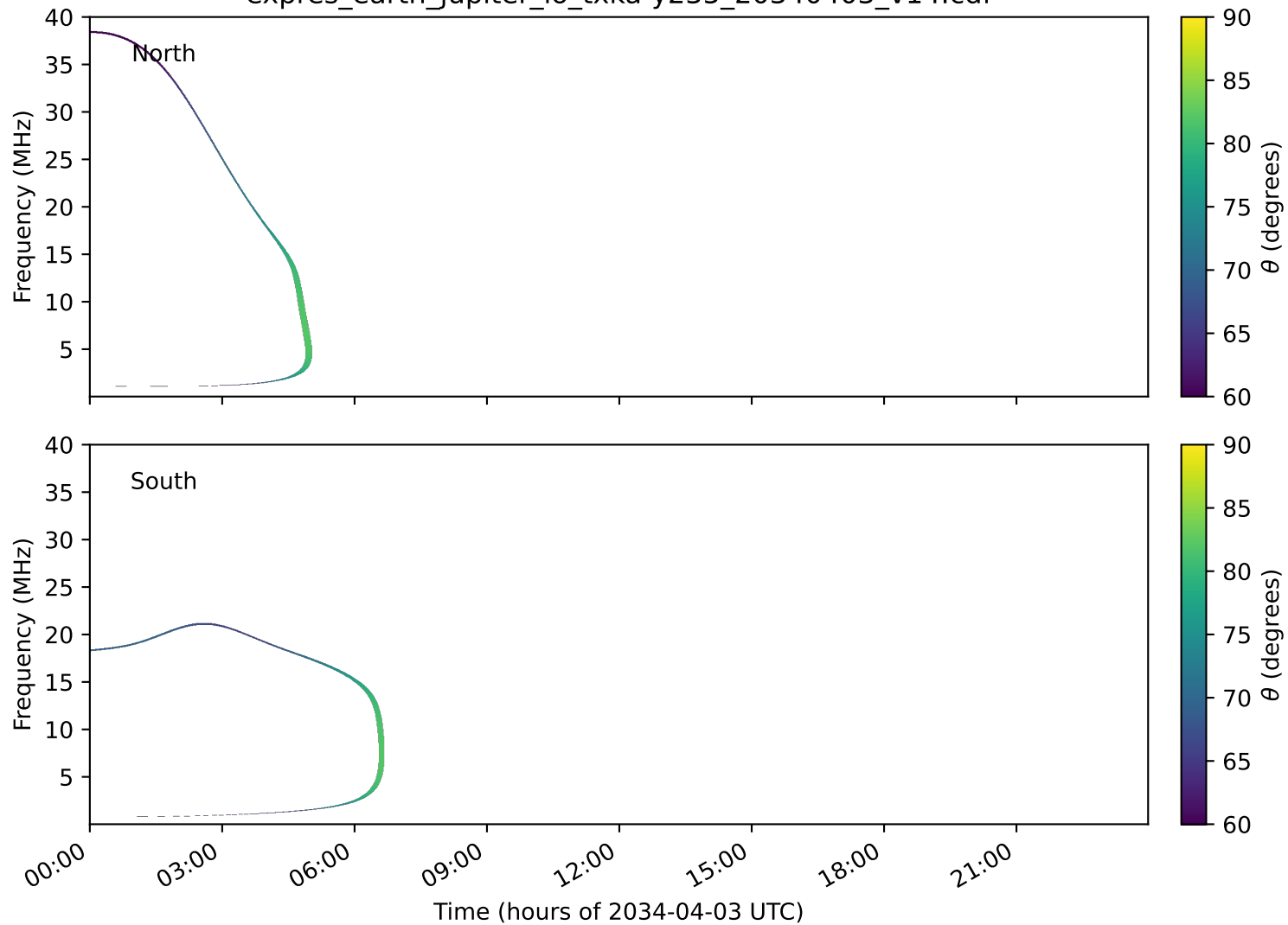
expres_earth_jupiter_io_txka-y235_20340403_v14.cdf
