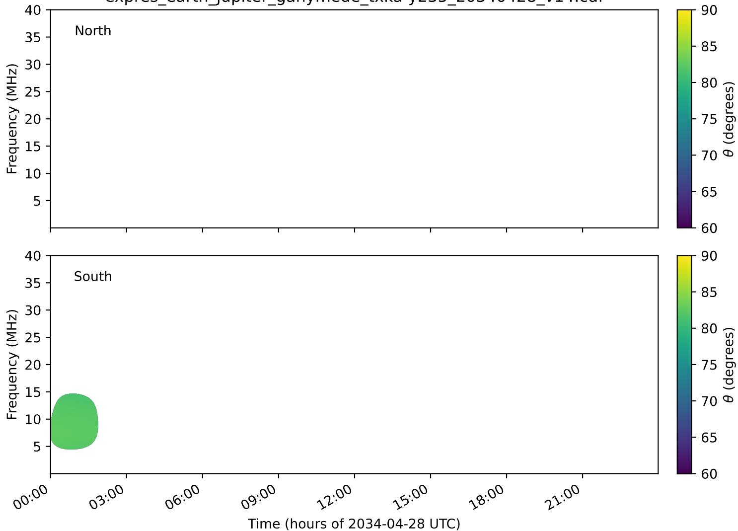
expres_earth_jupiter_ganymede_txka-y235_20340428_v14.cdf
