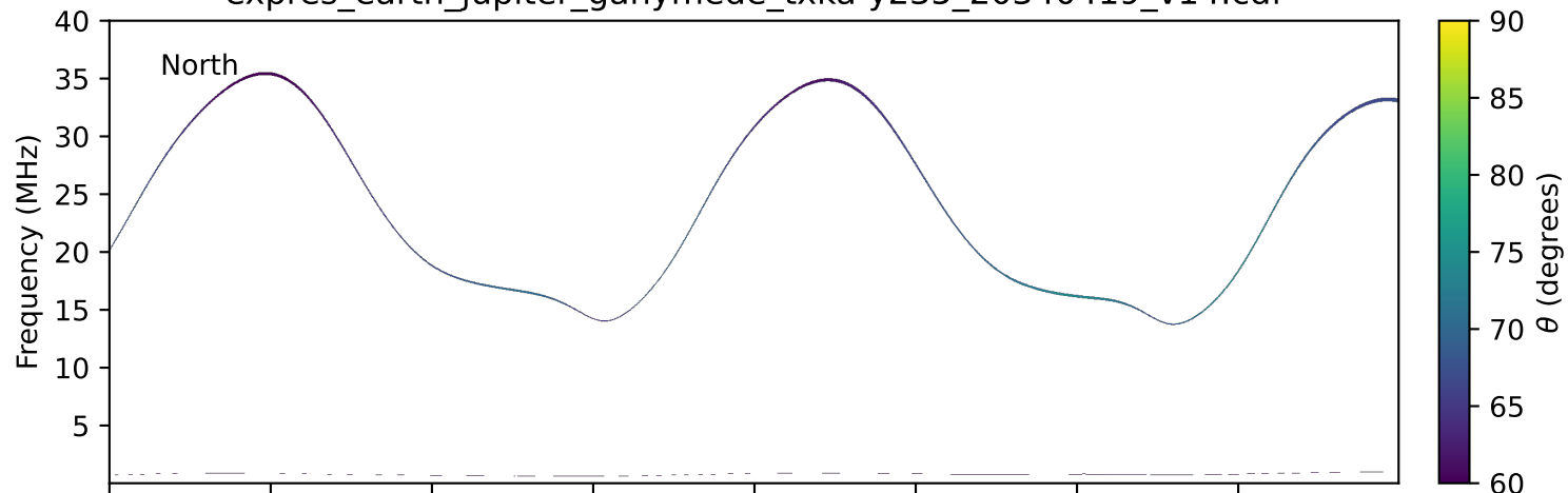
expres_earth_jupiter_ganymede_txka-y235_20340419_v14.cdf
