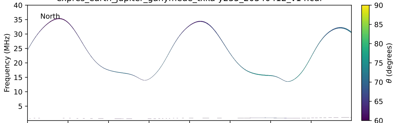
expres_earth_jupiter_ganymede_txka-y235_20340412_v14.cdf
