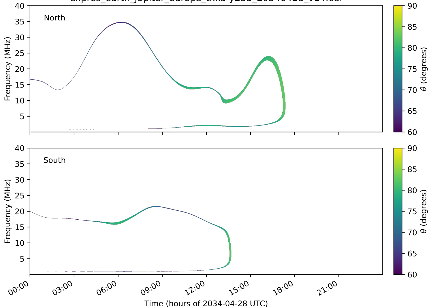
expres_earth_jupiter_europa_txka-y235_20340428_v14.cdf
