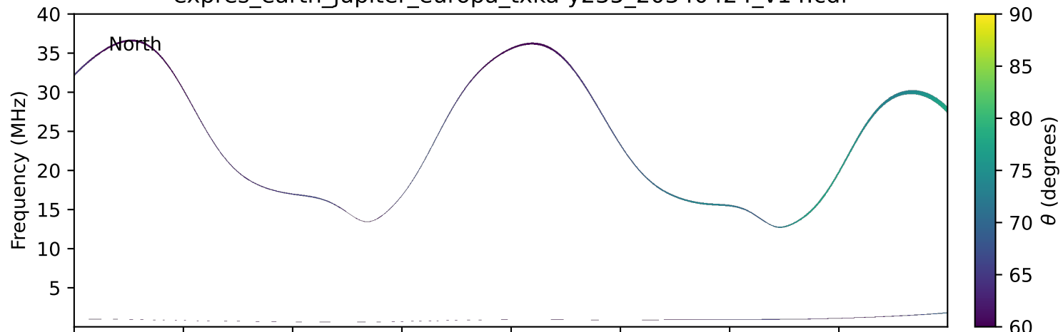
expres_earth_jupiter_europa_txka-y235_20340424_v14.cdf
