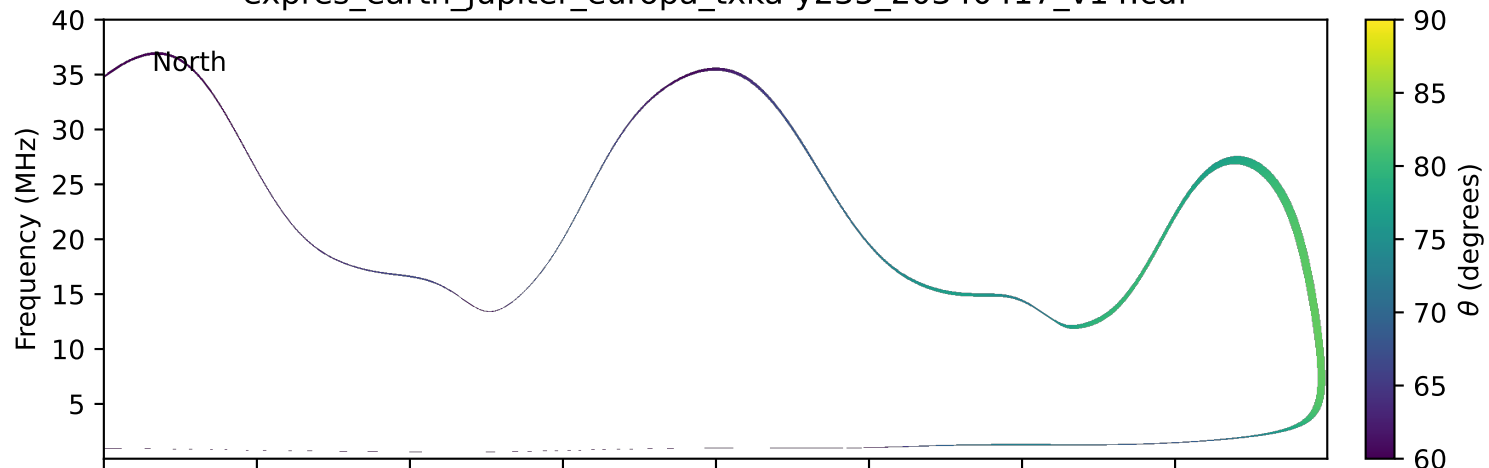
expres_earth_jupiter_europa_txka-y235_20340417_v14.cdf
