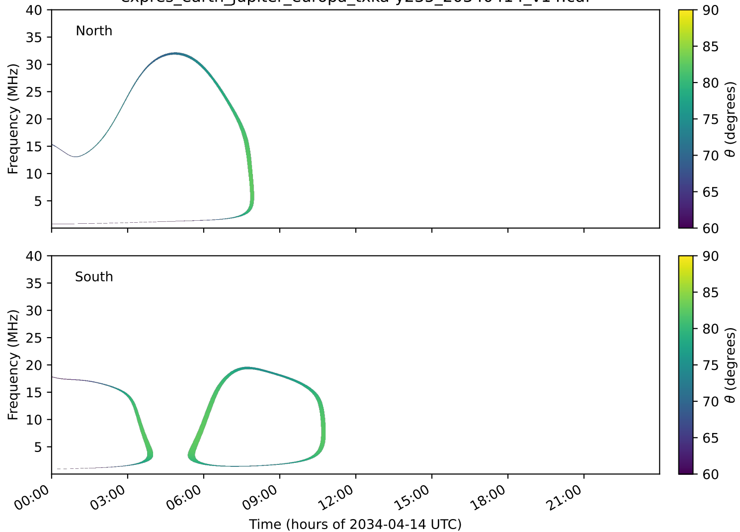
expres_earth_jupiter_europa_txka-y235_20340414_v14.cdf
