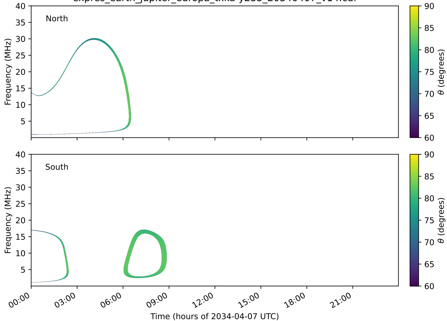
expres_earth_jupiter_europa_txka-y235_20340407_v14.cdf
