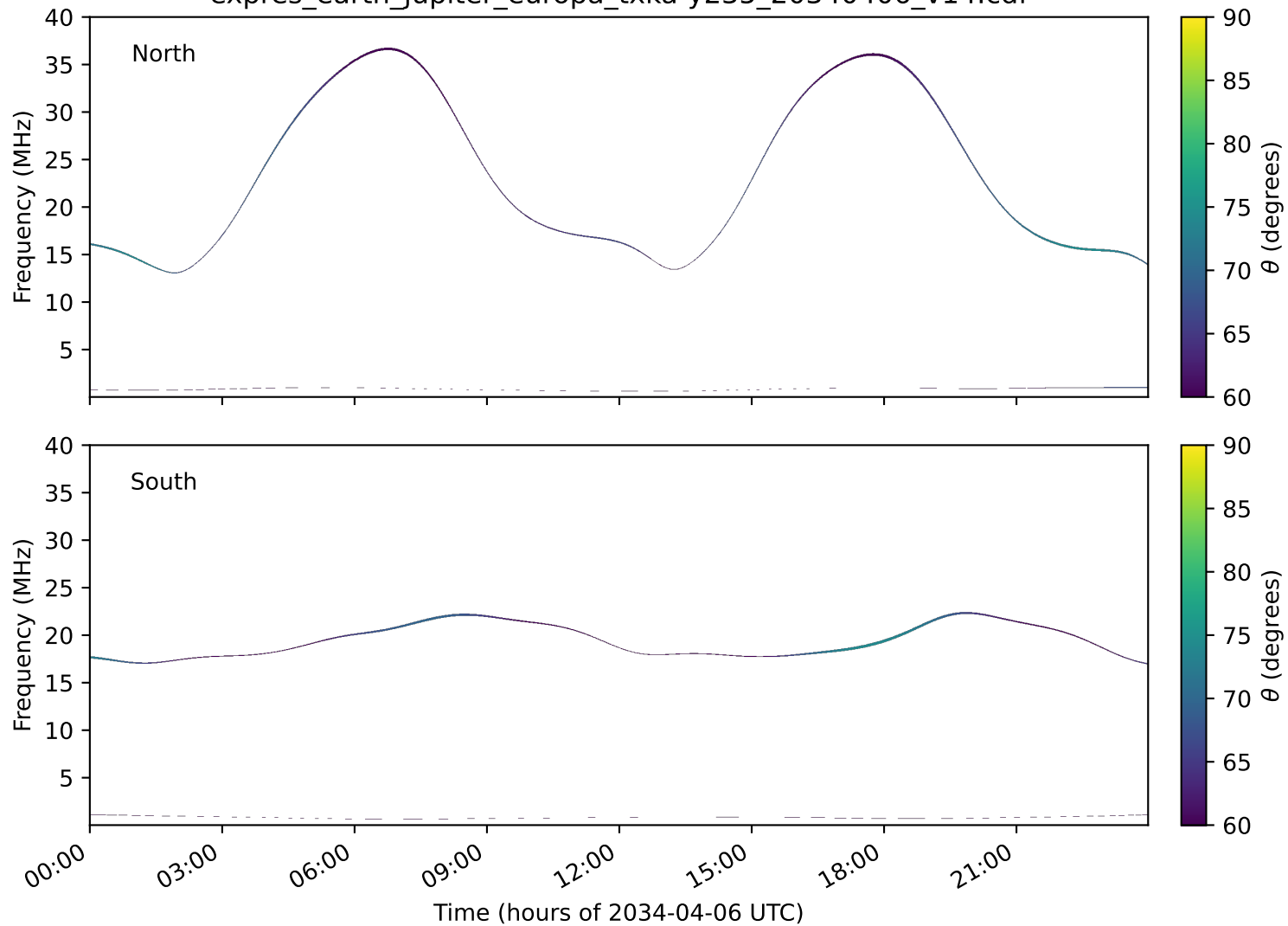
expres_earth_jupiter_europa_txka-y235_20340406_v14.cdf
