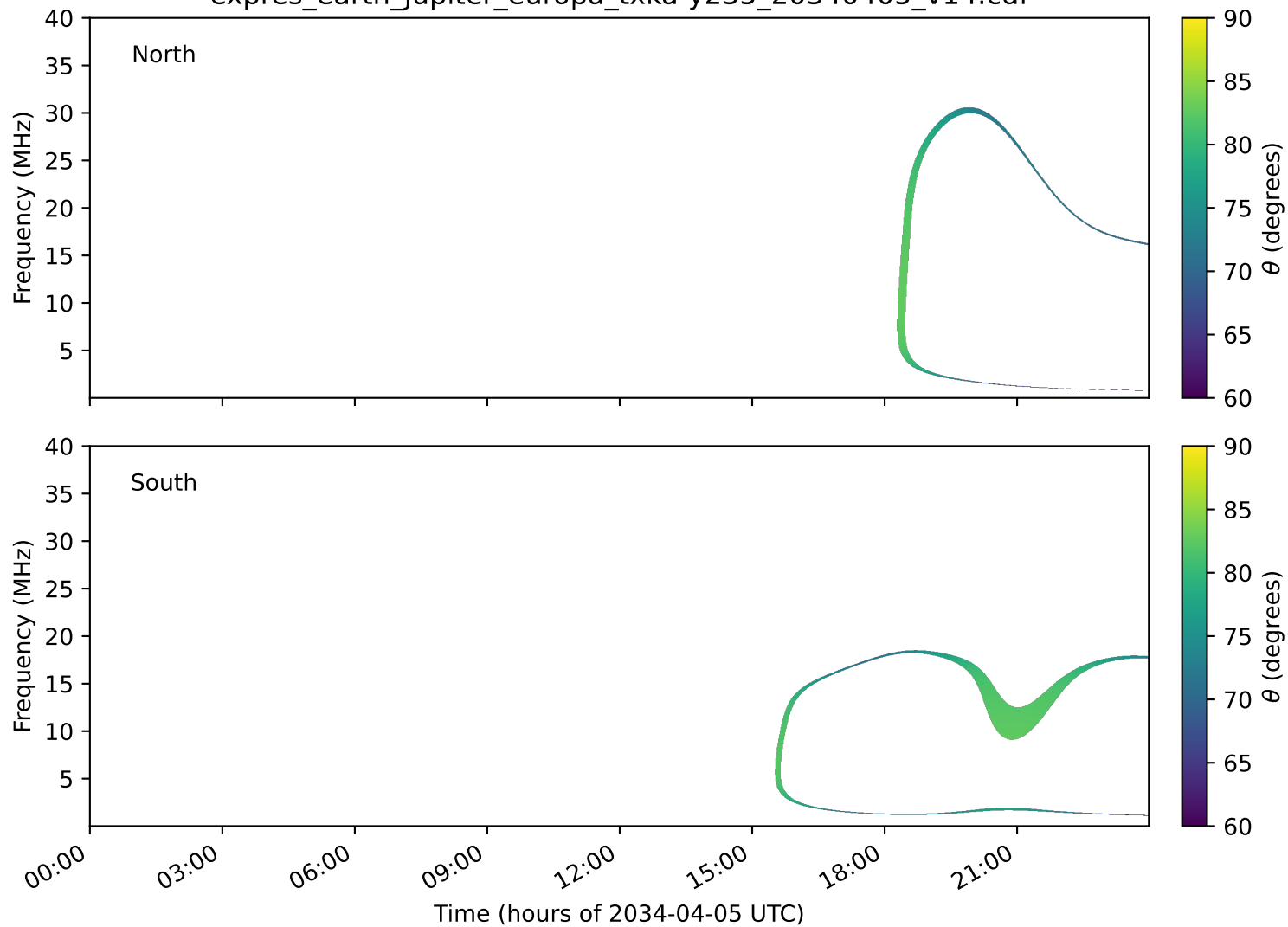
expres_earth_jupiter_europa_txka-y235_20340405_v14.cdf
