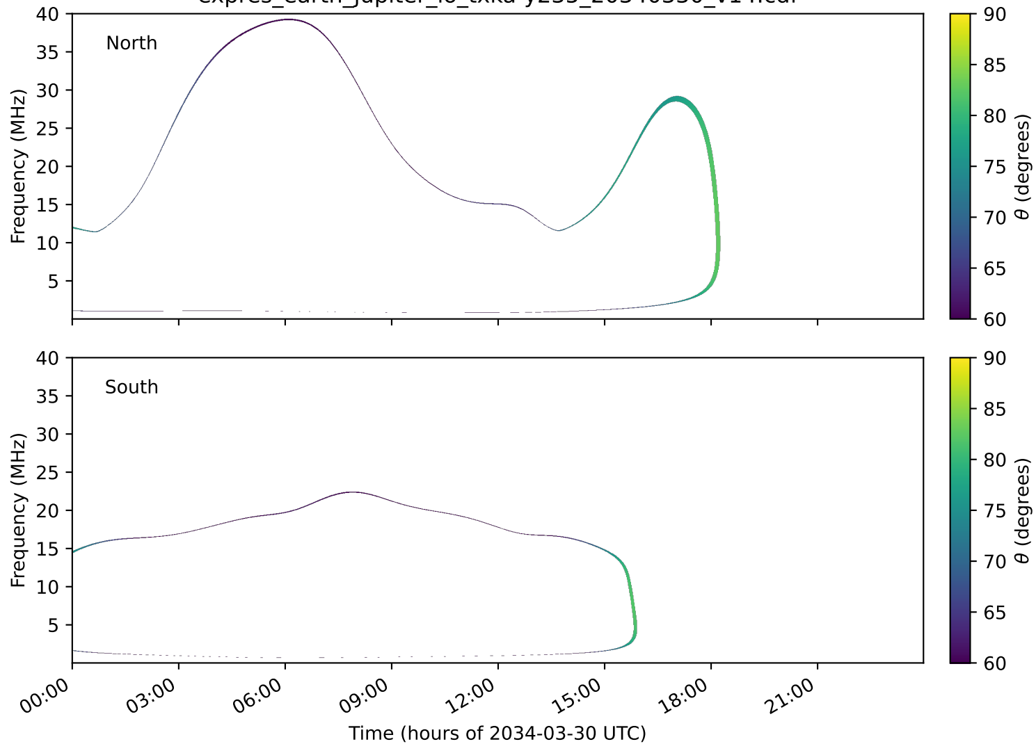
expres_earth_jupiter_io_txka-y235_20340330_v14.cdf
