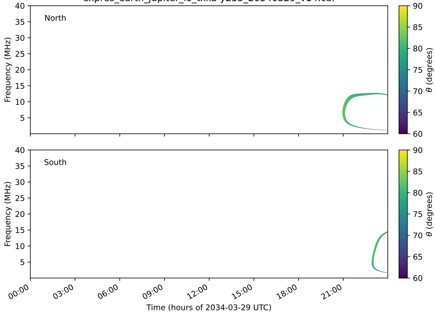
expres_earth_jupiter_io_txka-y235_20340329_v14.cdf
