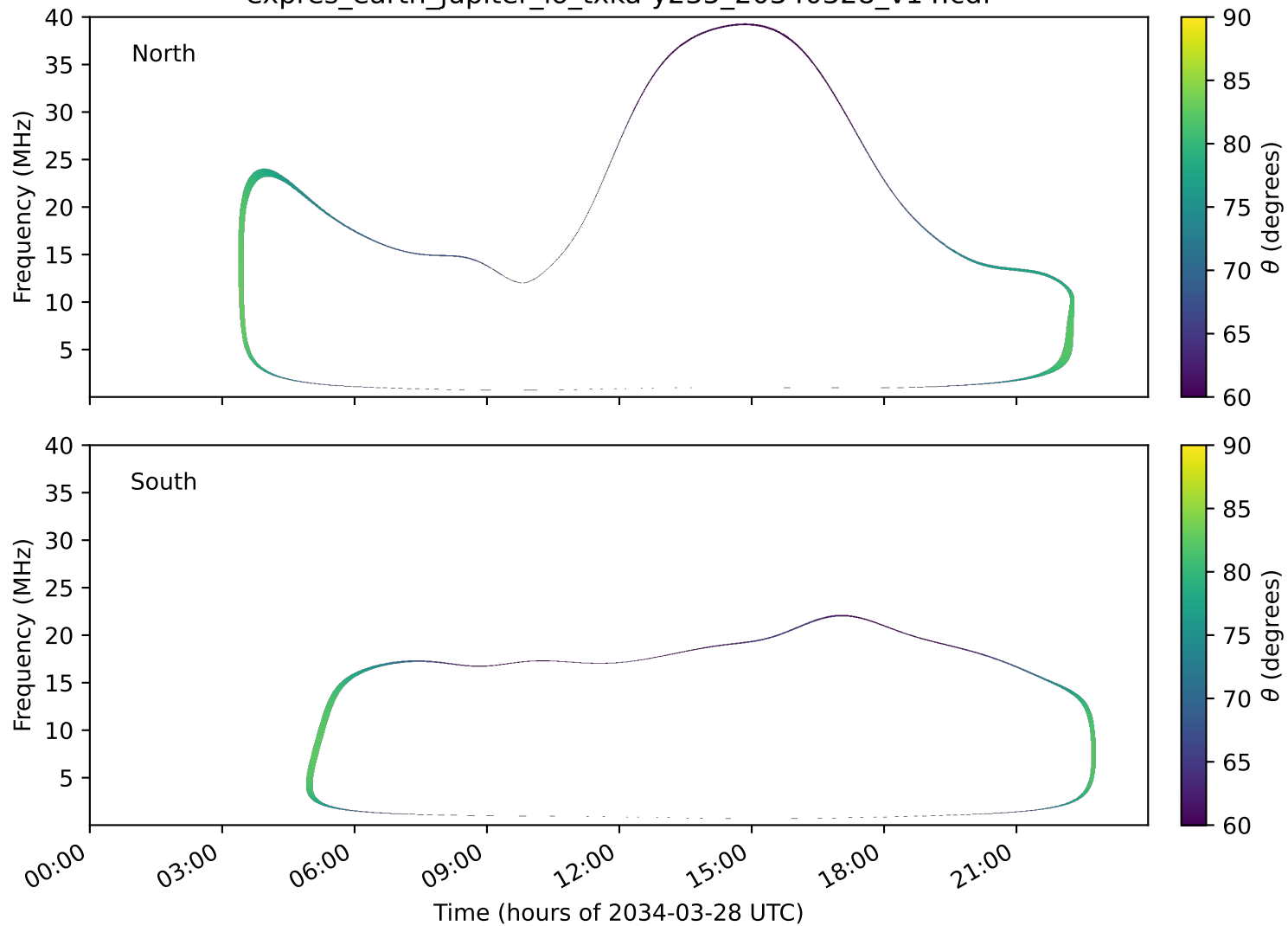
expres_earth_jupiter_io_txka-y235_20340328_v14.cdf
