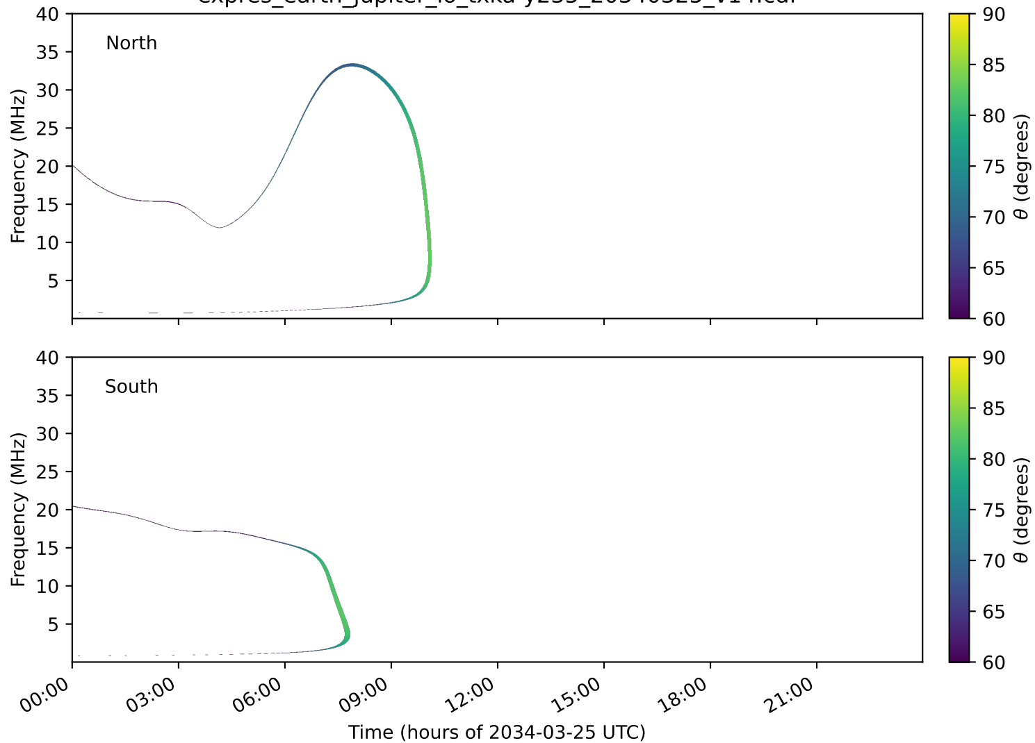
expres_earth_jupiter_io_txka-y235_20340325_v14.cdf
