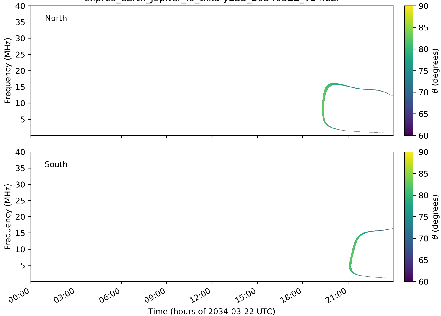
expres_earth_jupiter_io_txka-y235_20340322_v14.cdf
