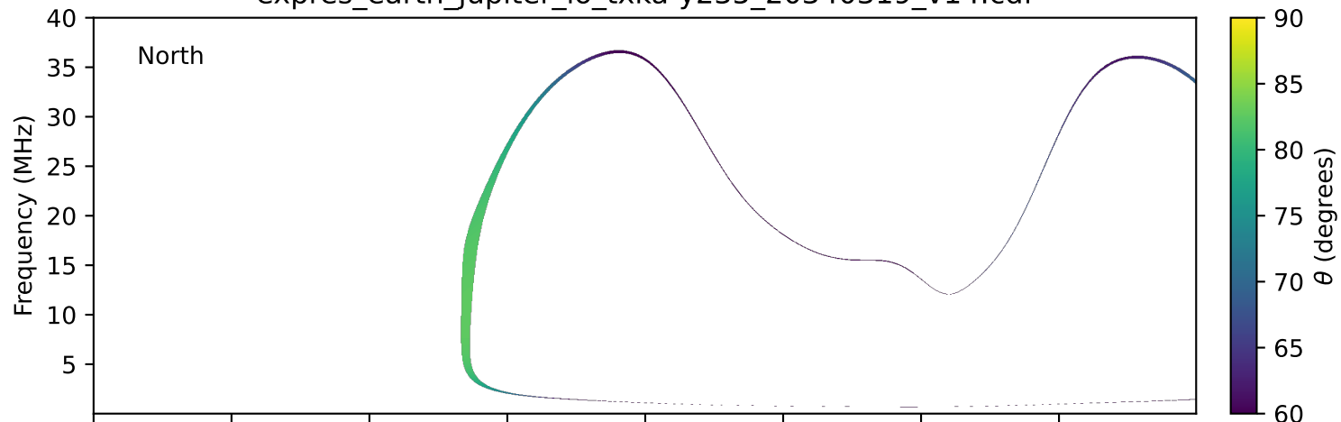
expres_earth_jupiter_io_txka-y235_20340319_v14.cdf
