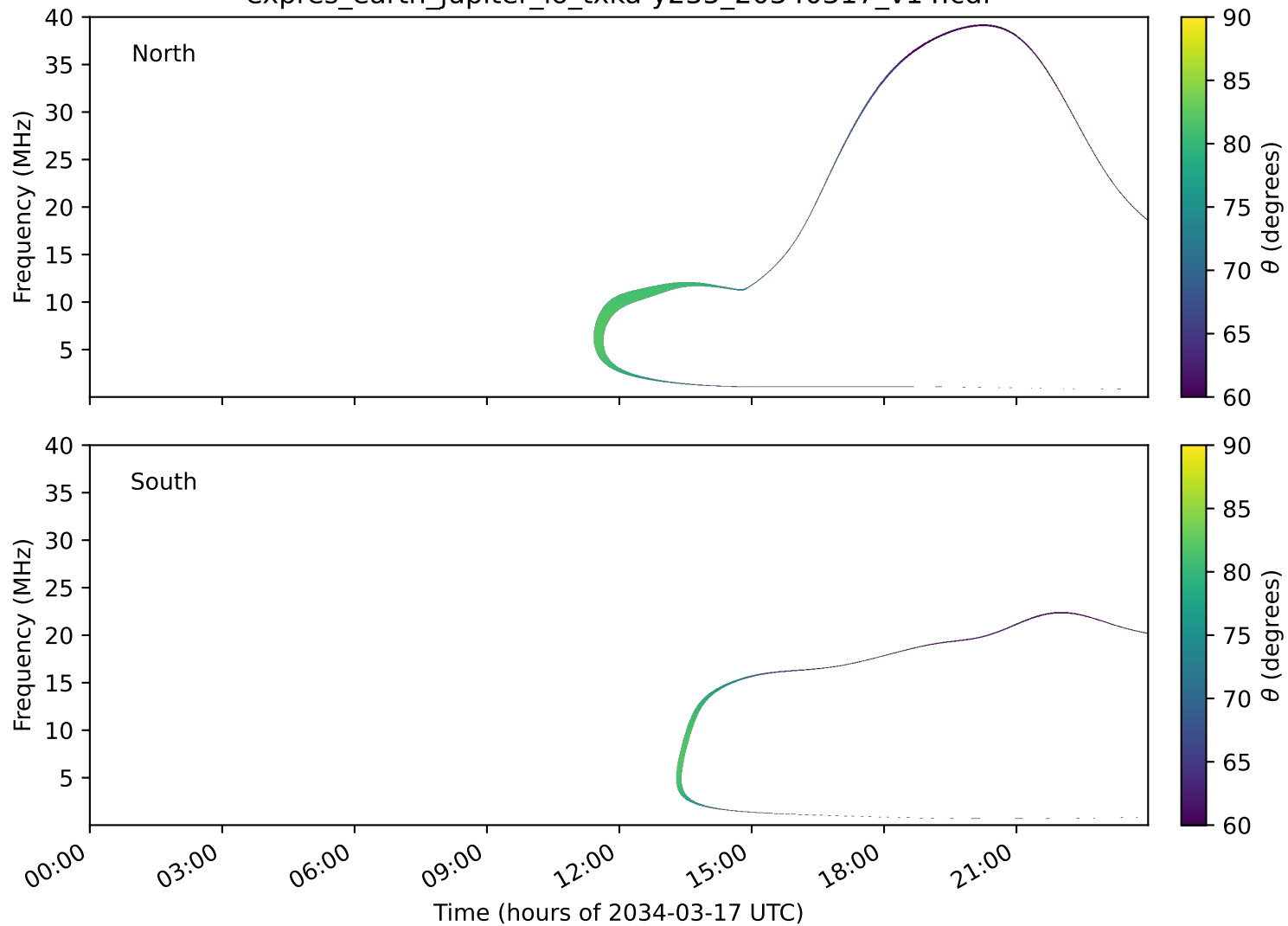
expres_earth_jupiter_io_txka-y235_20340317_v14.cdf
