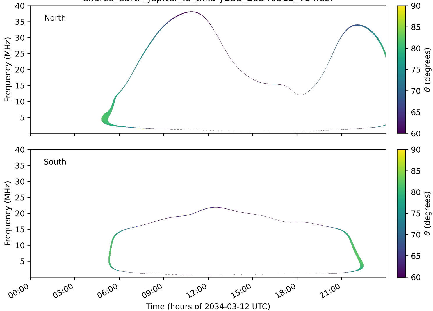
expres_earth_jupiter_io_txka-y235_20340312_v14.cdf
