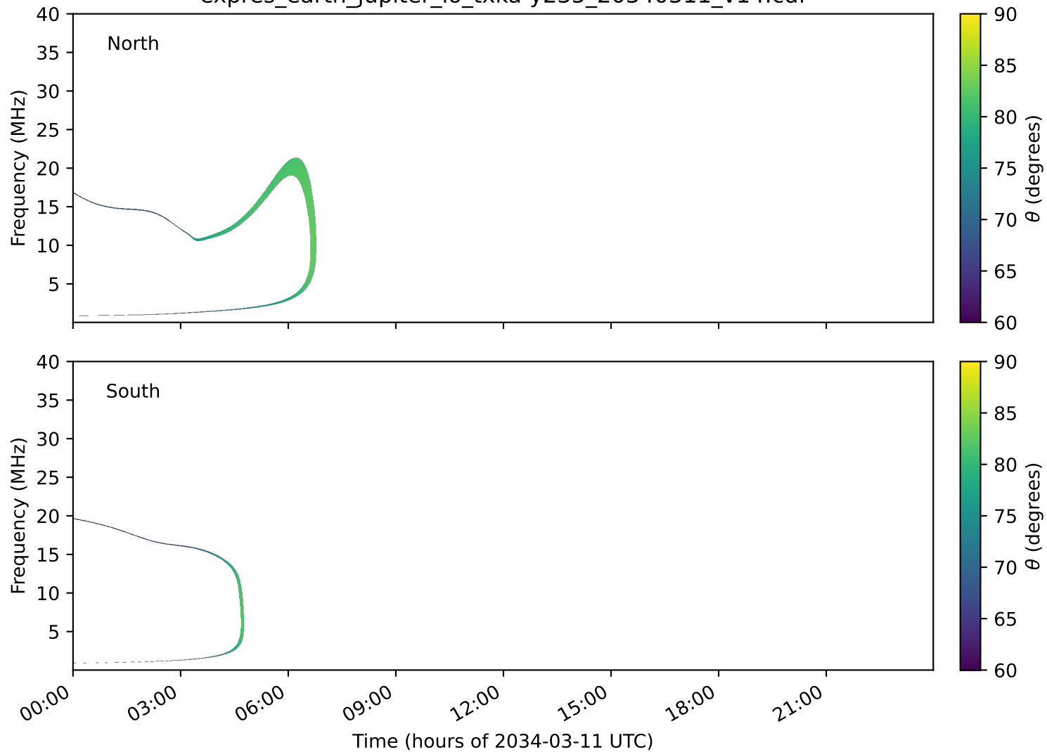
expres_earth_jupiter_io_txka-y235_20340311_v14.cdf
