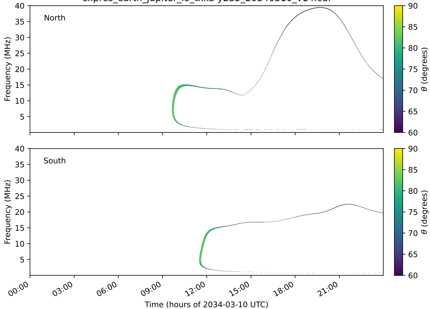
expres_earth_jupiter_io_txka-y235_20340310_v14.cdf
