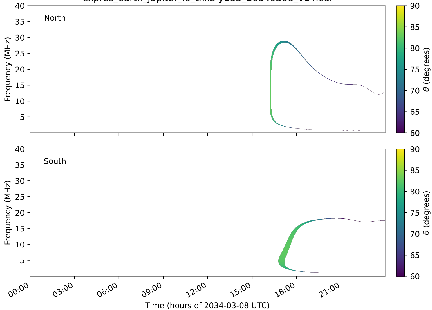
expres_earth_jupiter_io_txka-y235_20340308_v14.cdf
