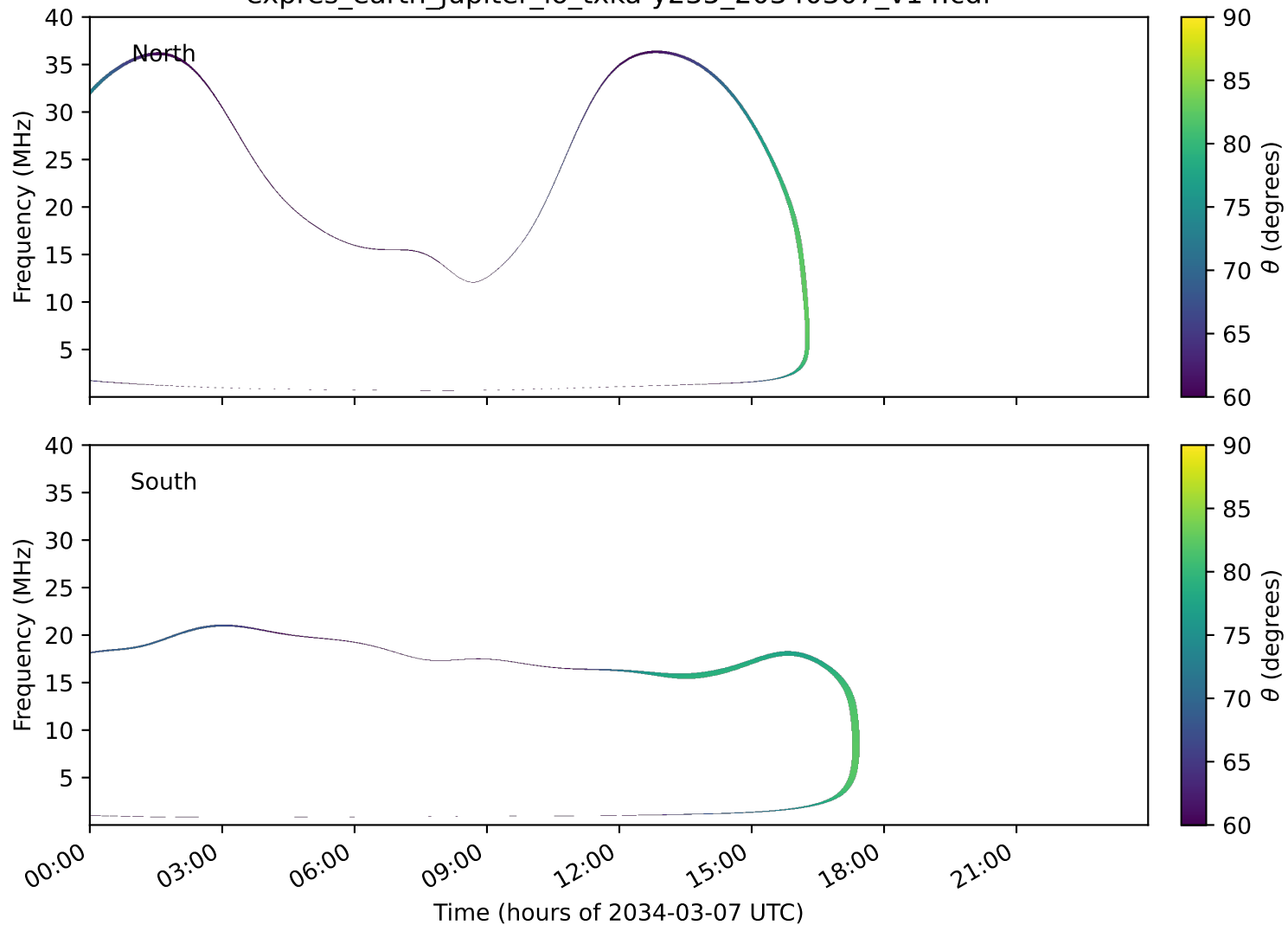
expres_earth_jupiter_io_txka-y235_20340307_v14.cdf
