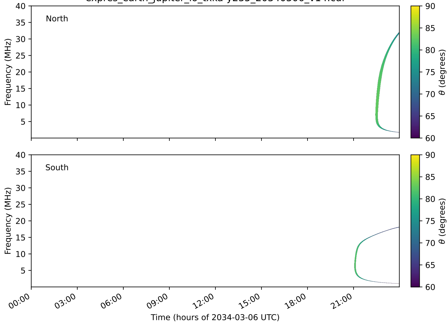
expres_earth_jupiter_io_txka-y235_20340306_v14.cdf
