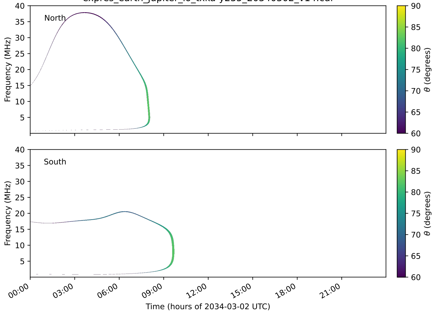
expres_earth_jupiter_io_txka-y235_20340302_v14.cdf
