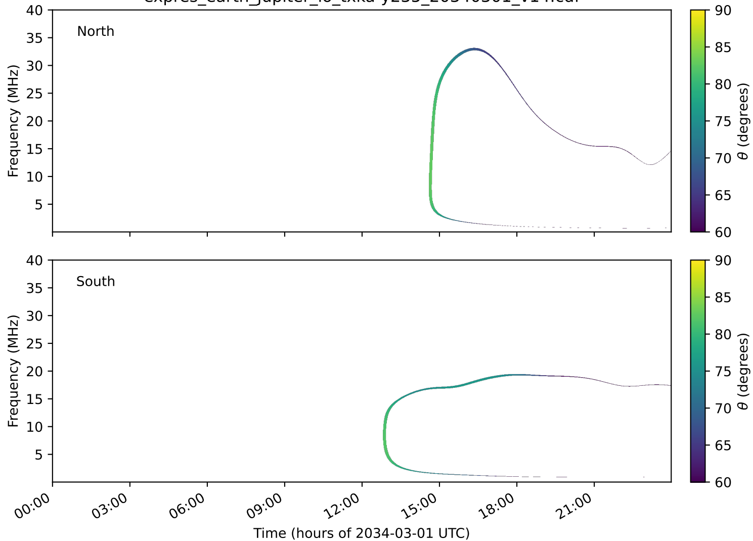
expres_earth_jupiter_io_txka-y235_20340301_v14.cdf
