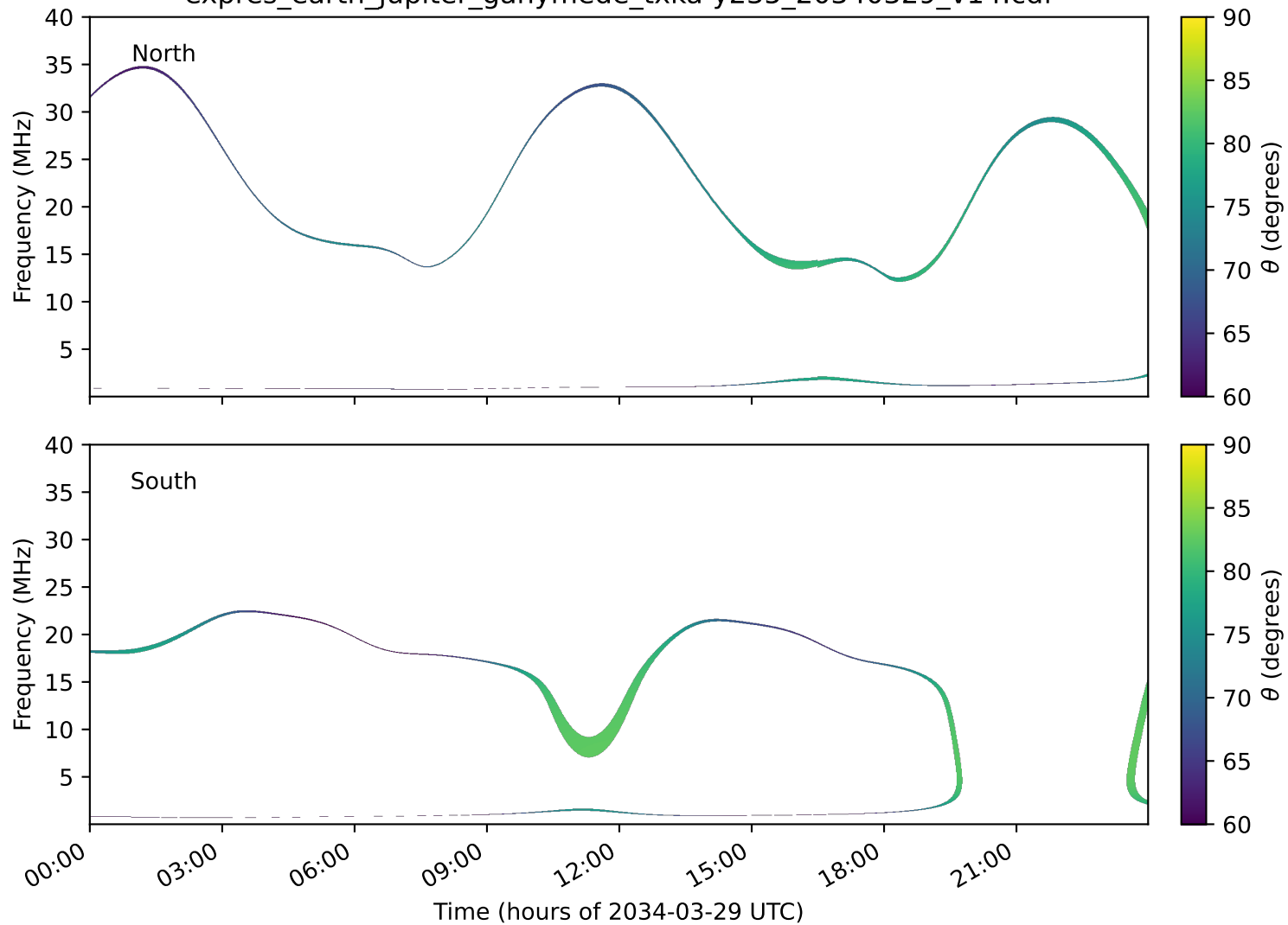
expres_earth_jupiter_ganymede_txka-y235_20340329_v14.cdf
