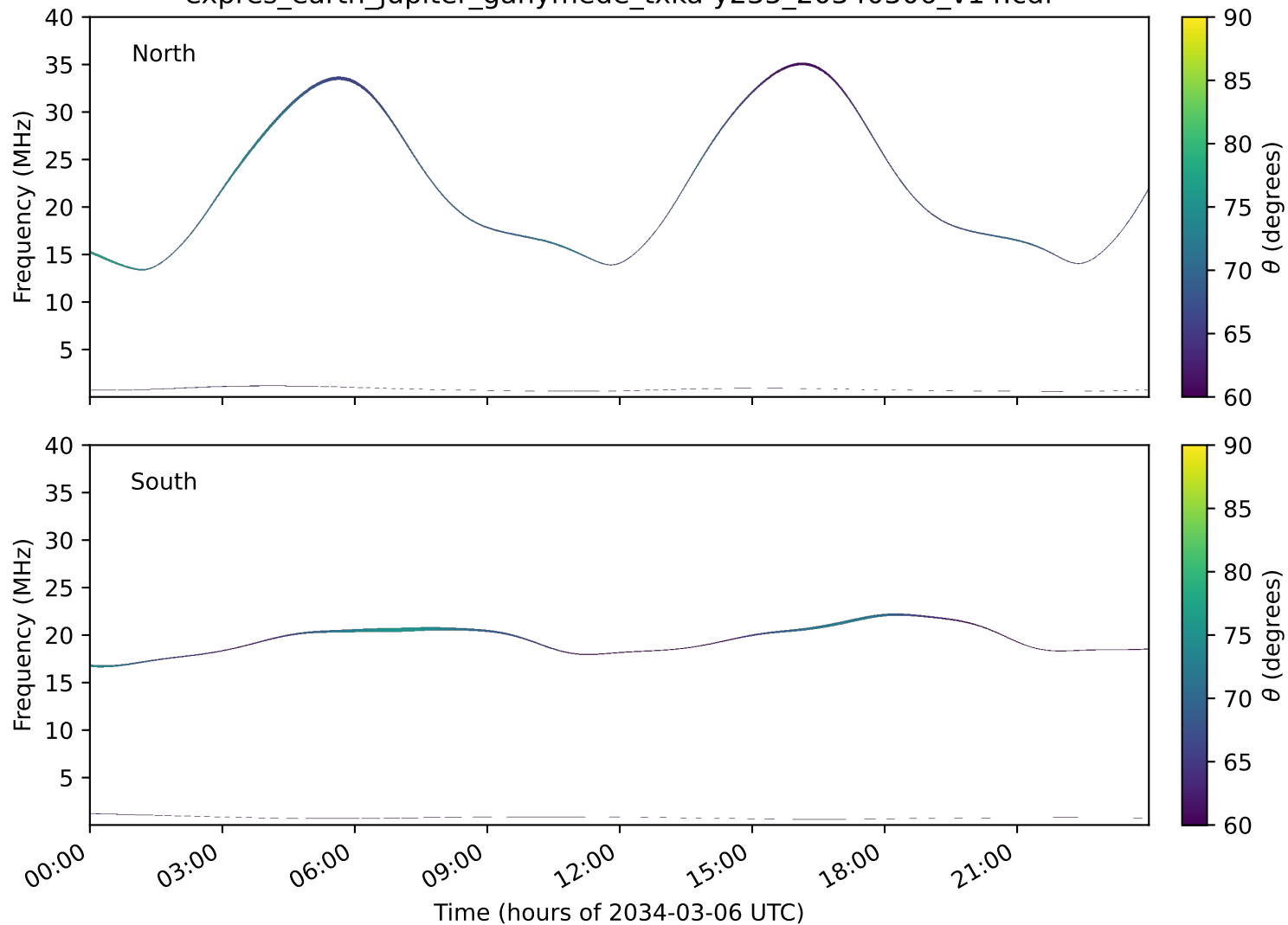
expres_earth_jupiter_ganymede_txka-y235_20340306_v14.cdf
