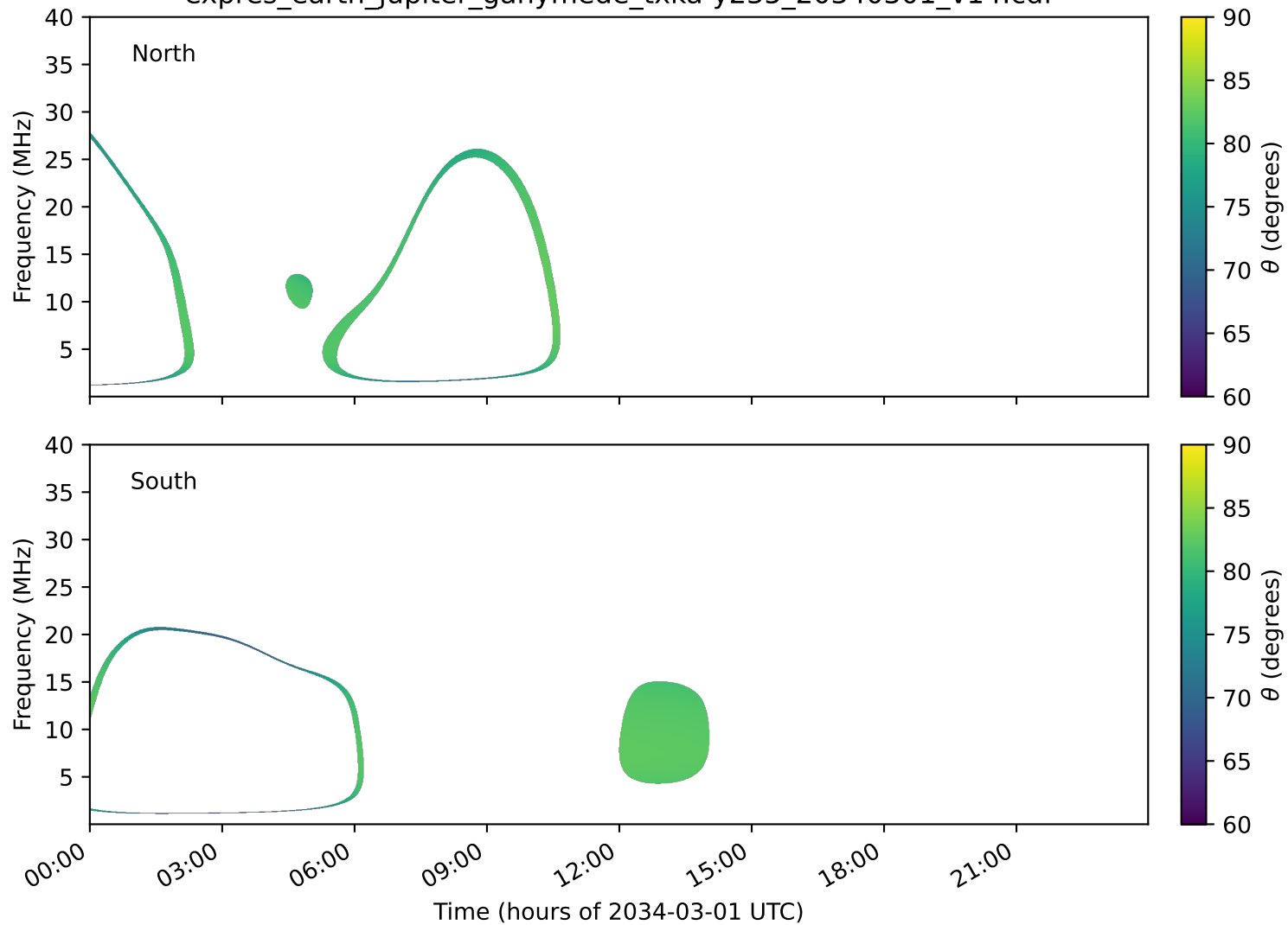
expres_earth_jupiter_ganymede_txka-y235_20340301_v14.cdf
