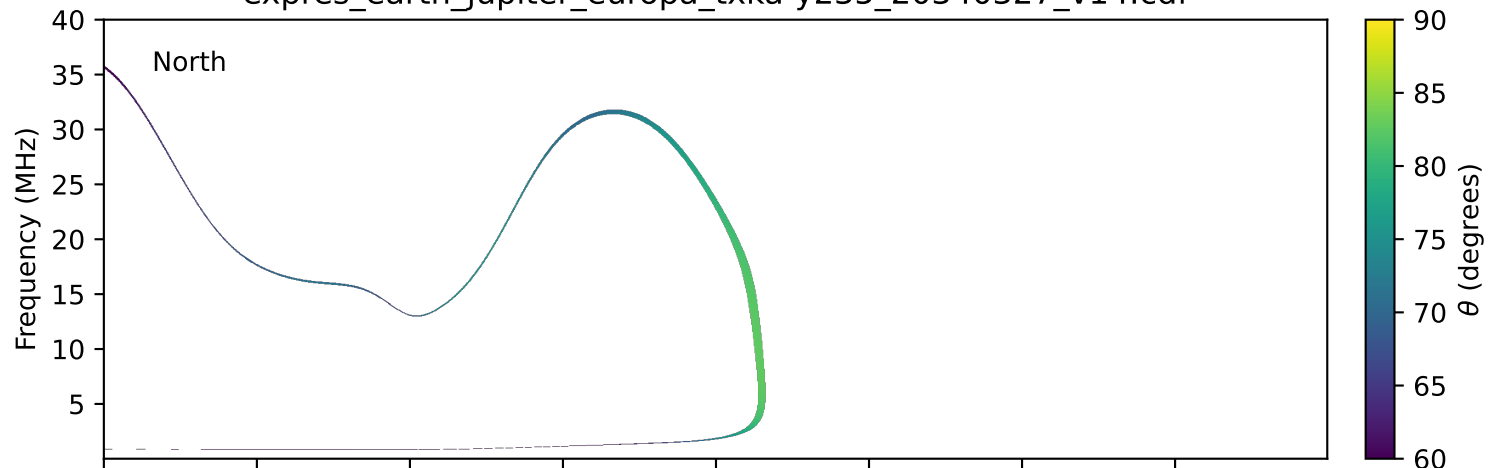
expres_earth_jupiter_europa_txka-y235_20340327_v14.cdf
